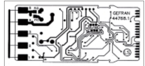
CPU BOARD
