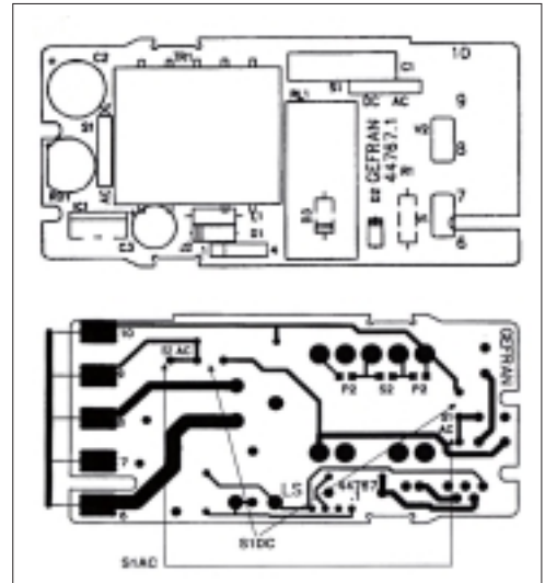
CPU BOARD
